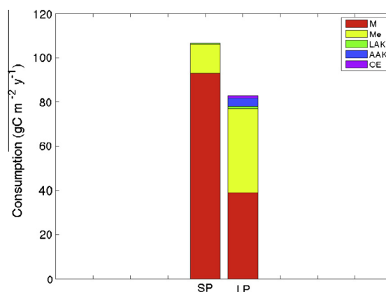
Fig. 3. Annual consumption ( \text{g C m}^{-2} \text{ y}^{-1} ) of large and small phytoplankton primary production by zooplankton groups obtained from the southwestern Antarctic Peninsula (sWAP) mass balance food web model. Phytoplankton groups are indicated as: small phytoplankton-SP and large phytoplankton-LP. Zooplankton groups are indicated as: mesozooplankton-Me; larval Antarctic krill-LAK; adult Antarctic krill-AAK; other euphausiids-OE.
