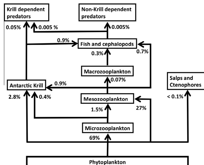
Fig. 6. Summary of the percent transfer of primary production between the pelagic components of the sWAP food web model.
