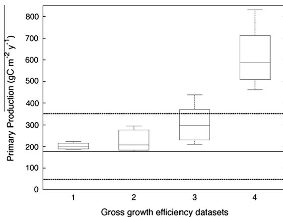
Fig. 7. Simulated estimates of primary production needed to support the south-western Antarctic Peninsula (sWAP) food web obtained using gross growth efficiency values; (1) calculated from production and assimilation efficiencies given in Table 1, (2) given in Banse (1995), (3) given in Priddle et al. (1998), and (4) derived from daily consumption rates (Table A.2). The boxes represent the range of the primary production estimates obtained from all of the simulations that used the indicated gross growth efficiencies. The median (horizontal line) and 25 and 75 percentiles (lower and upper vertical lines) are shown. The average ( 177 \text{ g C m}^{-2} \text{ y}^{-1} , solid line) and minimum and maximum ( 47 and 351 \text{ g C m}^{-2} \text{ y}^{-1} , dashed lines) primary production values estimated from field observations made on the sWAP continental shelf (Ducklow et al., 2007) are shown for comparison.
