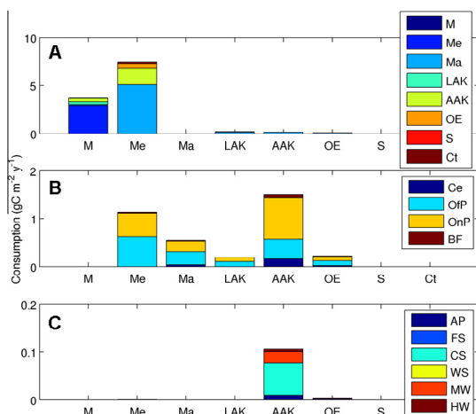
Fig. 4. Annual consumption ( \text{g C m}^{-2} \text{ y}^{-1} ) of zooplankton and benthic invertebrates by (A) zooplankton predators, (B) intermediate predators and (C) top predators calculated from the sWAP food web model. The species/groups are defined in Table 1.
