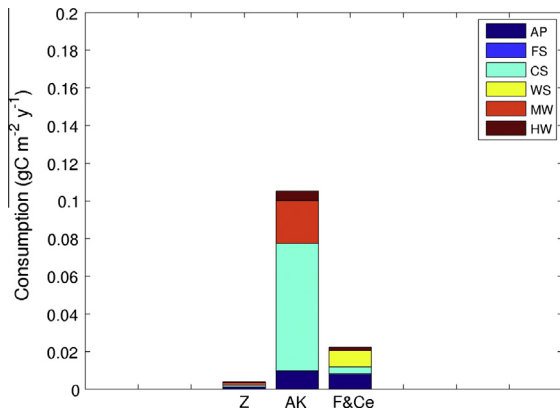
Fig. 5. Annual consumption ( \text{g C m}^{-2} \text{y}^{-1} ) of zooplankton and intermediate predators by top predators calculated from the southwestern Antarctic Peninsula (sWAP) food web model. Zooplankton (Z) prey include herbivorous zooplankton, carnivorous zooplankton and other euphausiids. Antarctic krill (AK) prey includes larvae and adults. Intermediate predators (F&Ce) include cephalopods, off- and on-shelf pelagic fish, and benthic fish.
