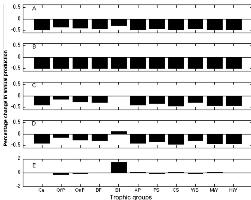
Fig. 8. Change in productivity, estimated relative to the reference simulation, of the southwestern Antarctic Peninsula (sWAP) higher trophic level components for (A) a 50% reduction in annual production of large phytoplankton; (B) a re-direction of 50% of small and large phytoplankton production from mesozooplankton, larval Antarctic krill, adult Antarctic krill, other euphasiids and salps to microzooplankton; (C) a redirection of 50% of large phytoplankton production from adult Antarctic krill to mesozooplankton; (D) a redirection of 50% of large phytoplankton production from adult Antarctic krill to salps; (E) a redirection of 50% of small and large phytoplankton production from mesozooplankton to salps. The bars (left to right) indicate changes in intermediate predators (cephalopods-Ce, off-shelf pelagic fish-OfP, on-shelf pelagic fish-OnP, benthic fish-BF), benthic invertebrates-BI, and top predators (Adélie penguin-AP, flying seabirds-FS, crabeater seals-CS, Weddell seals-WS, minke whales-MW, humpback whales-HW).
