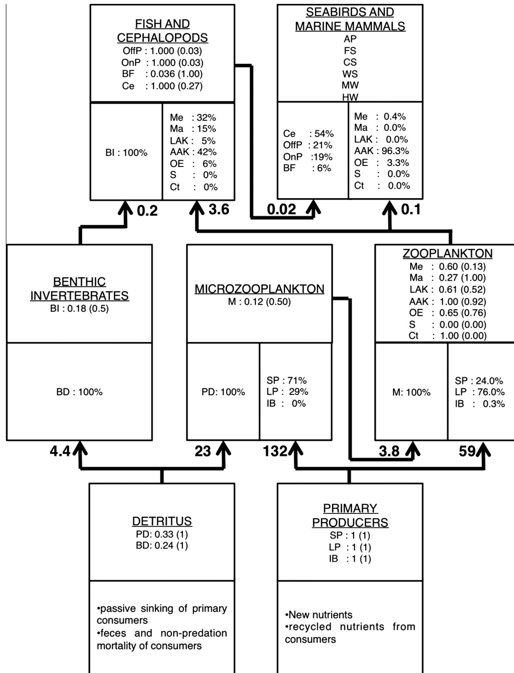
Fig. 2. Summary of the energy flows in the southwestern Antarctic Peninsula (sWAP) food web model. The 24 food web model groups are grouped into 7 compartments that correspond to primary producers, detritus, zooplankton, microzooplankton, benthic invertebrates, fish and cephalopods (intermediate predators), seabirds and marine mammals (top predators). Arrows indicate the transfer of energy between compartments ( \text{g C m}^{-2} \text{y}^{-1} ); the percentage contribution of model groups to these energy fluxes is indicated (bottom part of each box). For each model group, the overall proportion of annual production consumed in the food web (ecotrophic efficiency, first number, upper part of box) and the fraction of this proportion that is consumed outside the compartment (number in parentheses, upper part of box) is given. The species/groups are defined in Table 1.
